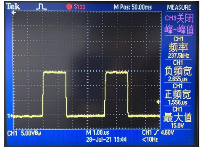
PWM waveform
